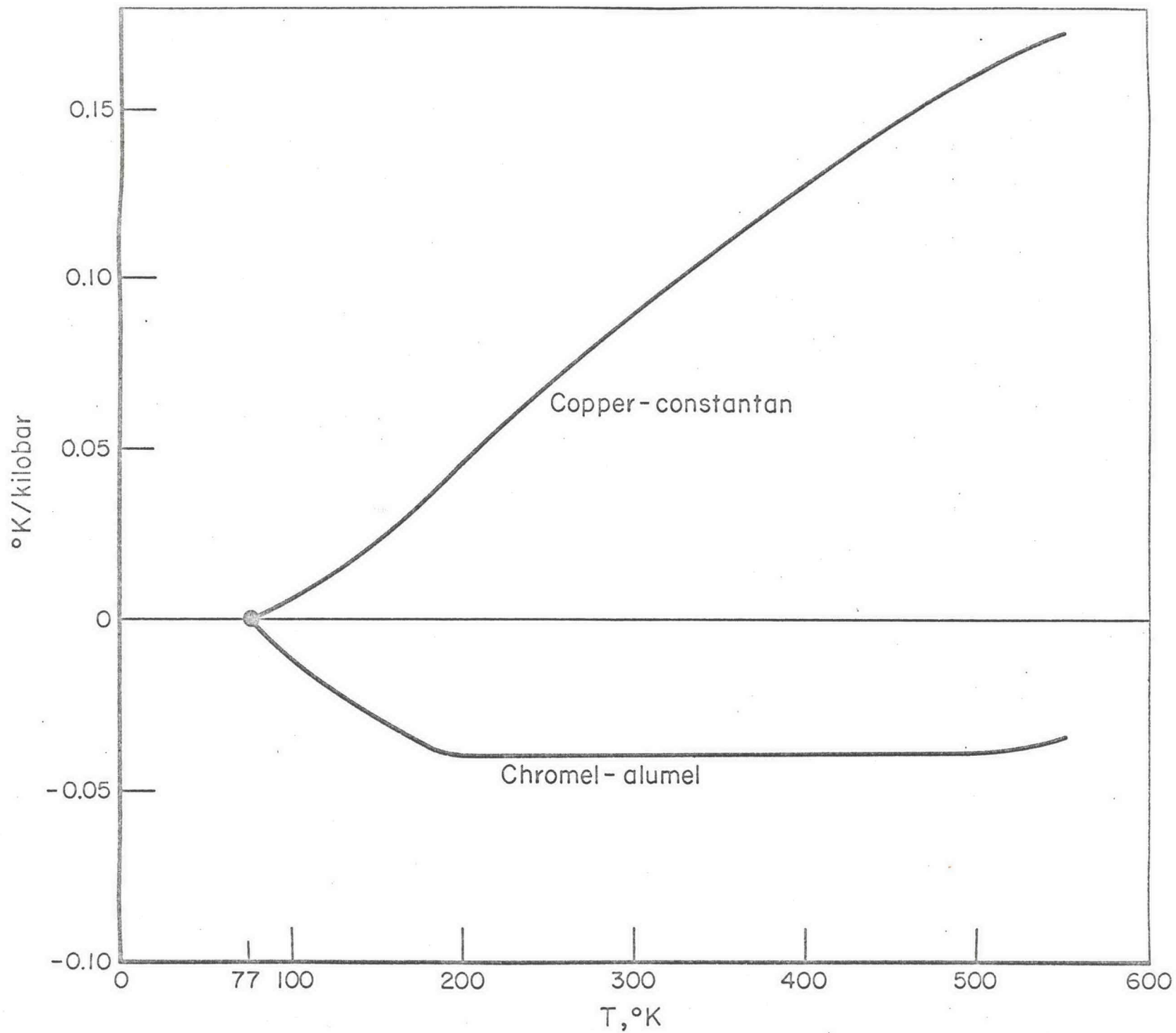
TEMPERATURE CORRECTION FOR PRESSURIZED THERMOCOUPLES Lead out at 78° K ; hot junction at T
